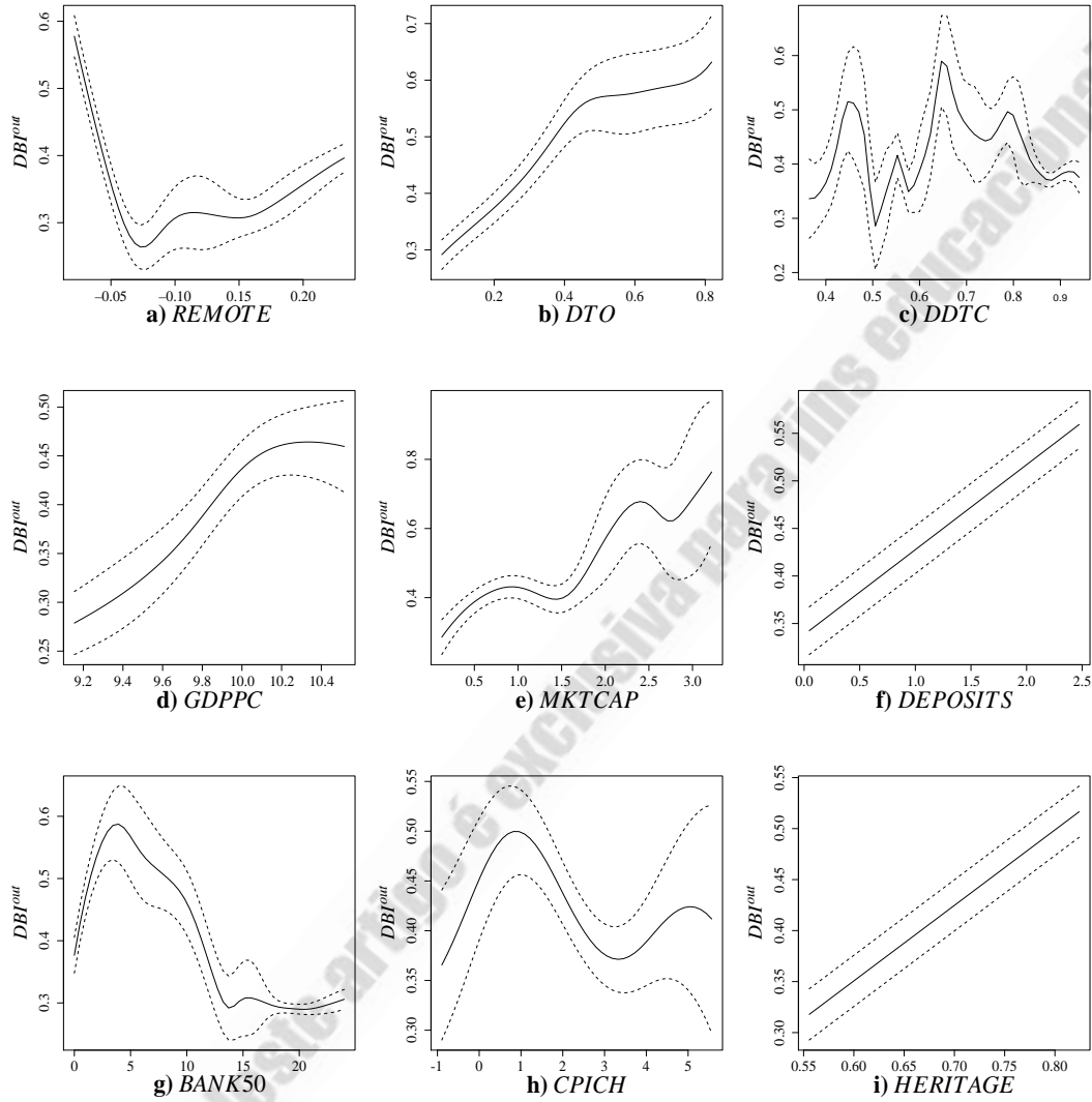
Figure 1: Nonparametric regression, DBI^{out}
